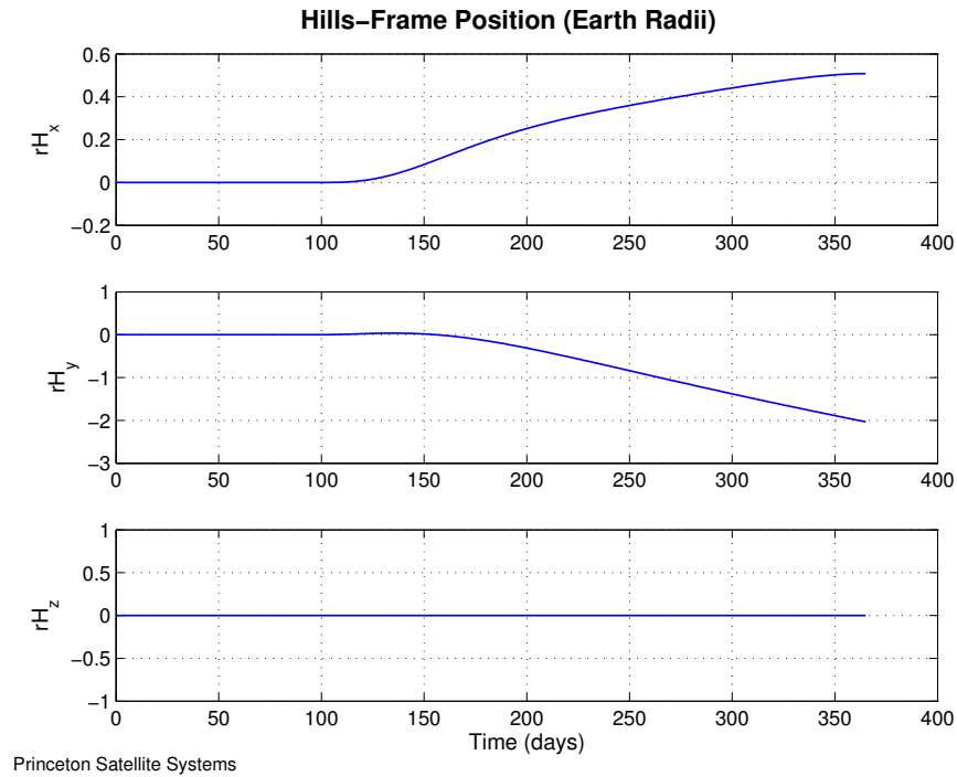
Figure 13. Optimal Hills-frame position history for the example deflection maneuver.
