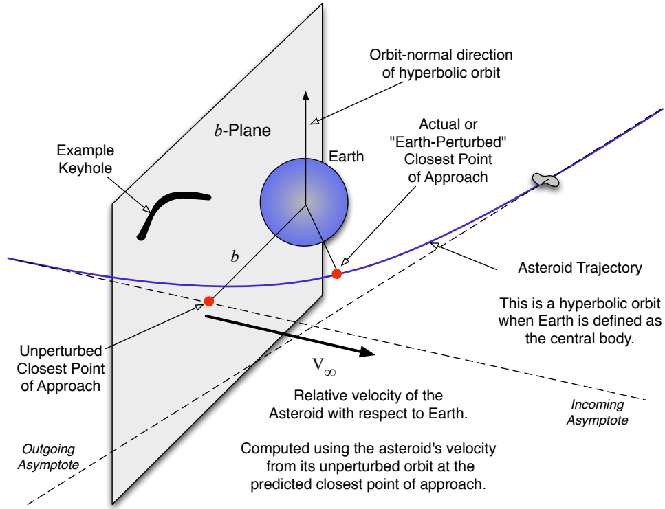
Figure 6. b -Plane Diagram. Illustrates the geometry of the encounter as the relative velocity vector intersects the b -Plane. The plane includes the line from Earth to the predicted closest point of approach, and it is perpendicular to the incoming asymptote.
