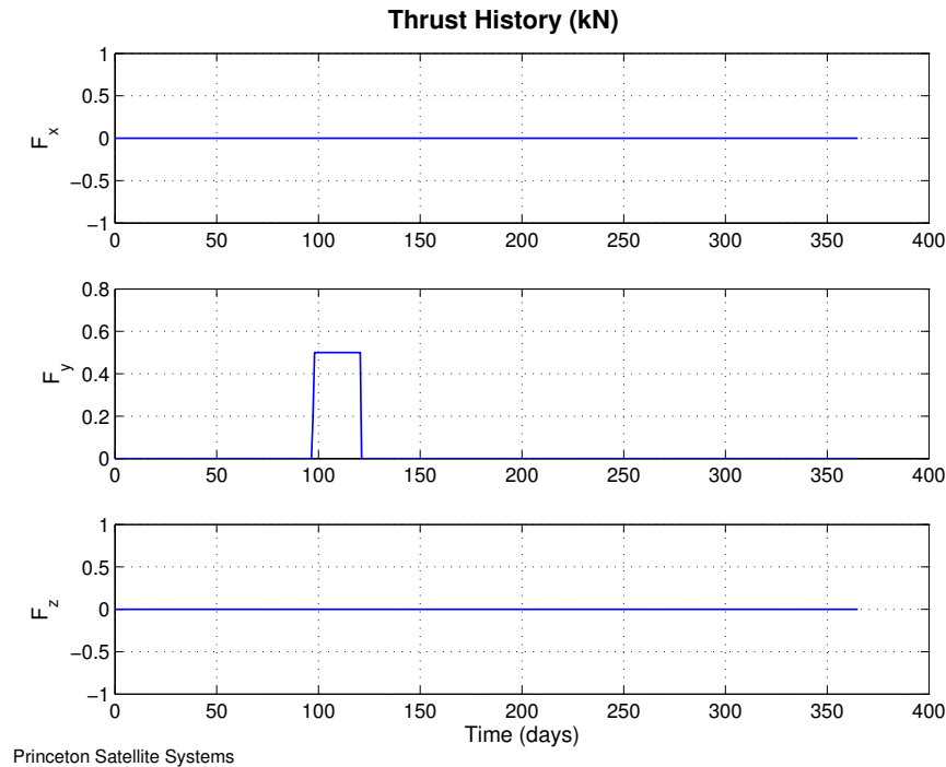
Figure 12. Optimal control history for the example deflection maneuver.
