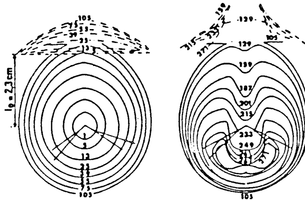
(b) Bubble No. 23: R_{\max}/l_0 = 0.95 , time scale: 8 \times 10^{-5} s.
