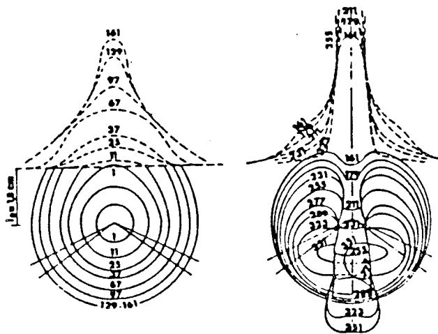
(c) Bubble No. 25: R_{\max}/l_0 = 1.5 , time scale: 8 \times 10^{-5} s.
