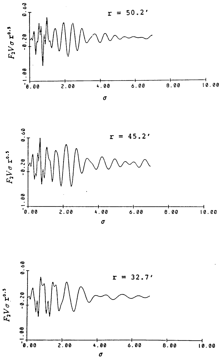
Figure 3-4. Imaginary parts of the transform of records collected at three different locations.
