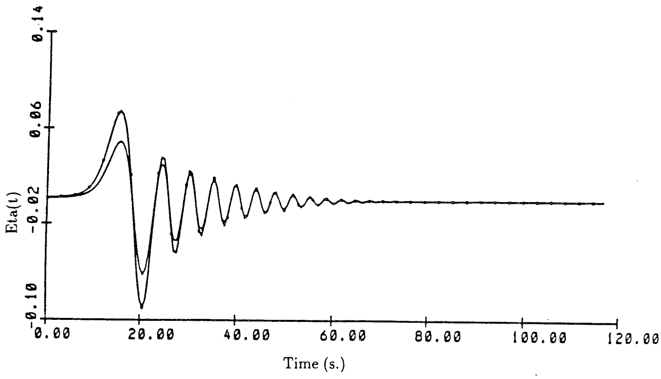
Figure 7-3. Comparison of wave records for a 'dome' initial condition of \hat{\eta}_{\max} = 1 , and R_c = 3 . The bottom slope S = 1/20 . The dotted curve is the solution on slope at r = 15 from GZ, while the smooth curve is the solution on a flat bottom.
